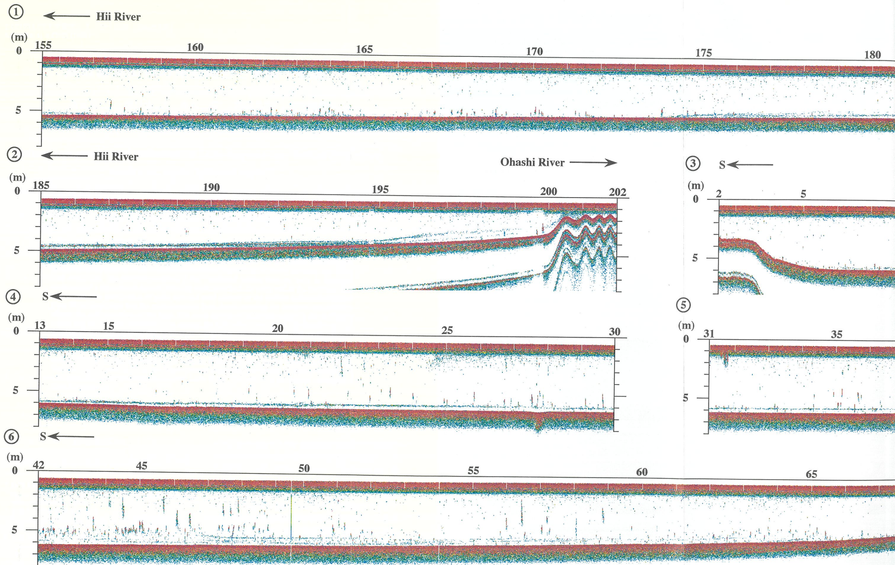
Fig. 11 Echo-sounding digital records along the tracks (E-W and N-S) surveyed on Feb. 26, 1993 in Lake Shinji
