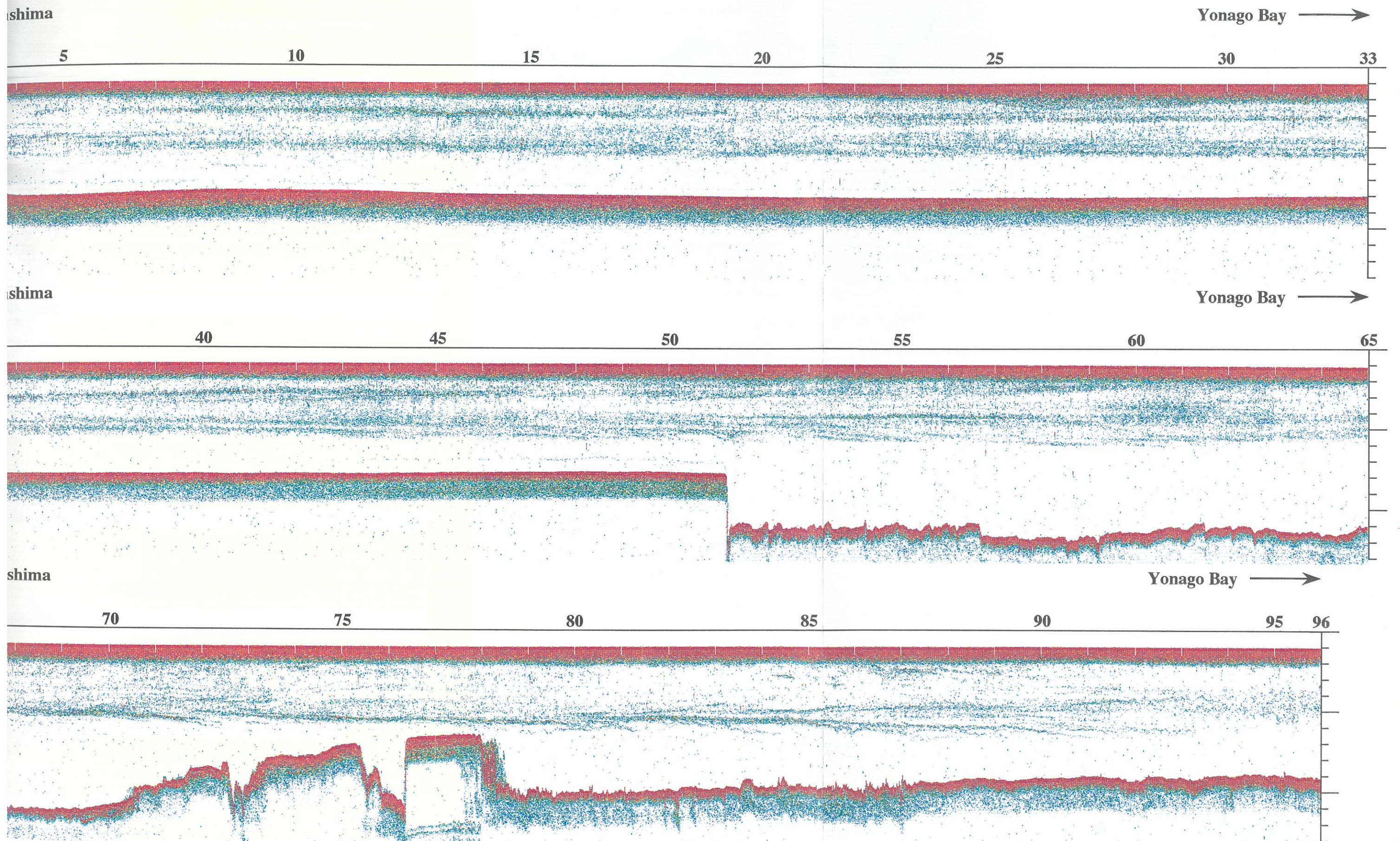
Fig. 10 Echo-sounding digital records along the track surveyed on August 19, 1993 in Lake Nakaumi
