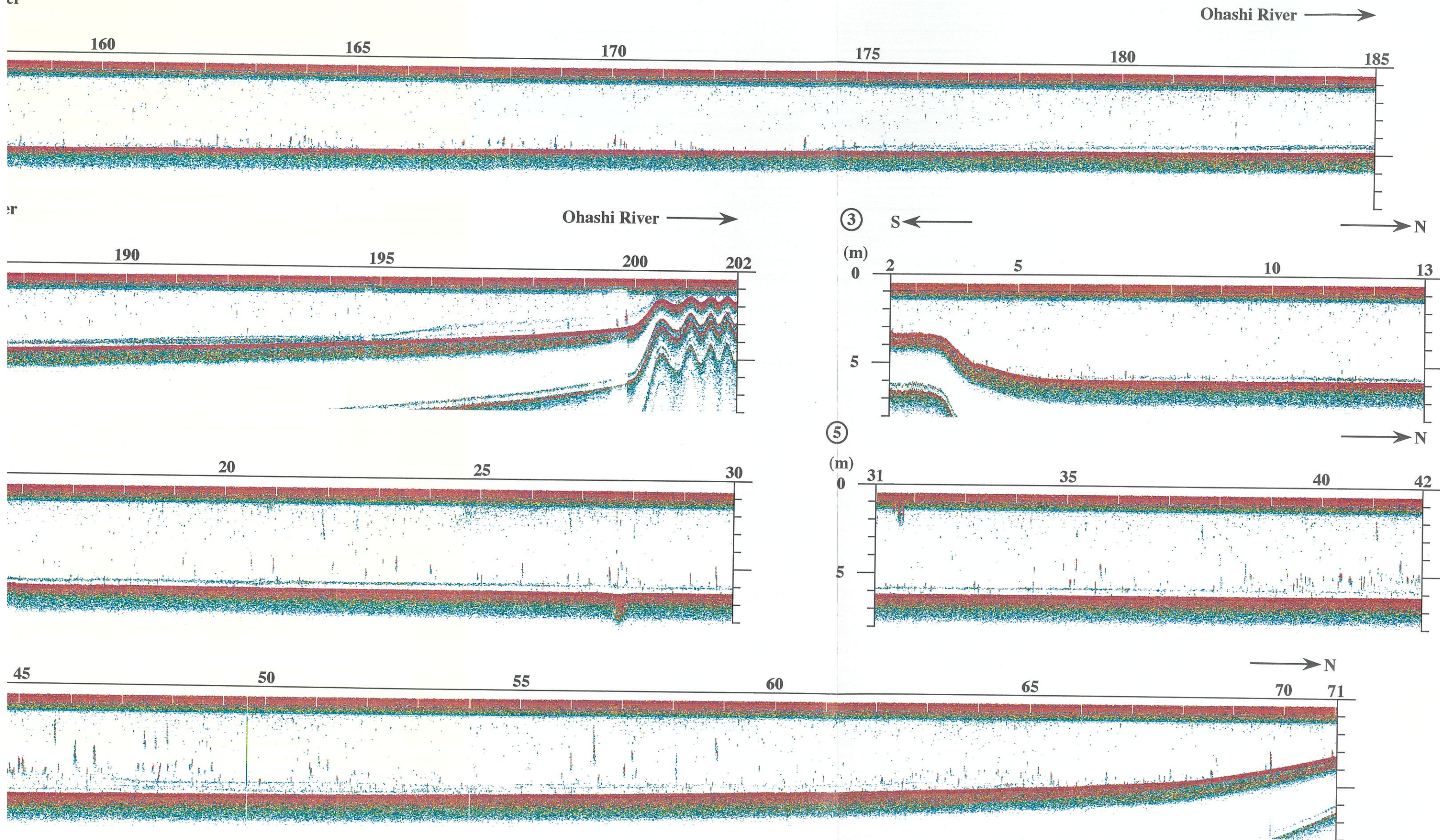
Fig. 11 Echo-sounding digital records along the tracks (E-W and N-S) surveyed on Feb. 26, 1993 in Lake Shinji
